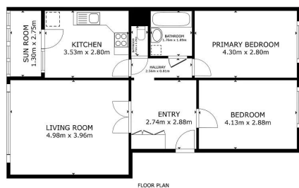
FLOOR PLAN
